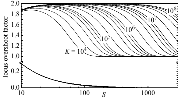
Figure 9. For the first oscillation mode, we compare the Richardson velocity overshoot in both magnitude and location over a wide spectrum of physical parameters half way across the channel. To the accuracy of the graph, predictions from (5.31) and (8.2) are indistinguishable.
