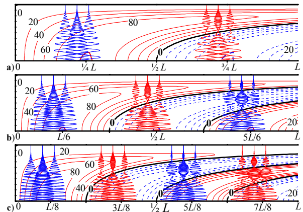
Figure 4. Evenly spaced iso-vorticity lines shown in (a), (b) and (c) for the first three harmonics when S = 25m and K = 10^6 m . The oscillatory velocity u_1 is abbreviated by four evenly spread timelines depicted at select locations coinciding with harmonic pressure nodes.
