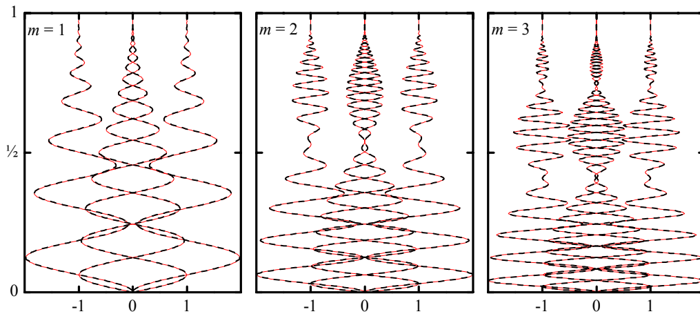
Figure 2. A plot of u_1 versus y at four successive times separated by a \pi/2 phase difference. For every oscillation mode, profiles are depicted at the last harmonic pressure node, where x/l = (2m-1)/2m . Here S = 25m and K = 10^6 m . To the accuracy of the graph, asymptotics (full lines) and numerics (broken lines) are indistinguishable.
