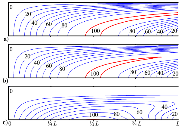
Figure 3. Evenly spaced iso-vorticity lines shown in (a), (b) and (c) for S = 10, 20 and 100 . In all cases, m = 1 and K = 10^6 . This variation can be ascribed to an order of magnitude depreciation in wall injection.
