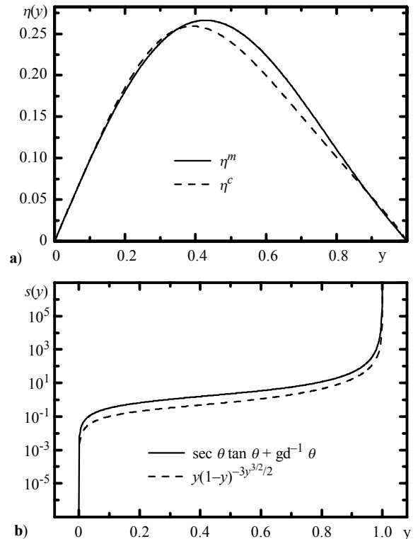
Figure 7. Comparing the effective scale functional \eta in (a) and corresponding scale function s in (b) to existing composite scale results given by Majdalani [38]. Superscripts refer to 'multiple' or 'composite' scale solutions.
