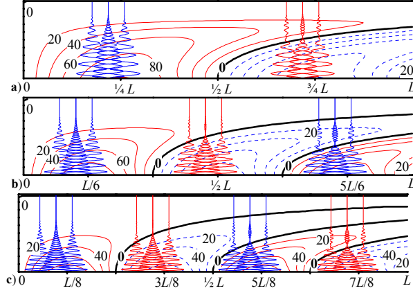
Figure 5. As in Fig. 4, unsteady velocity profiles overlay evenly spaced iso-vorticity lines in (a), (b) and (c) for the first three harmonics. Here K = 10^5 m , corresponding to an order of magnitude increase in kinematic viscosity. In the presence of surface injection, the penetration of rotationality is inhibited by viscous dissipation.
