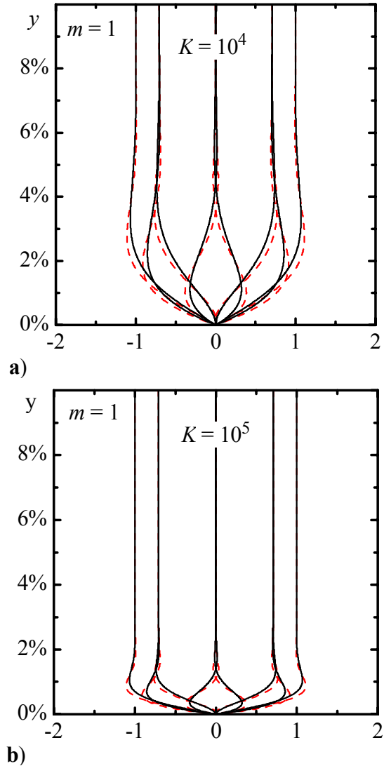
Figure 6. Velocity profiles of u_1 shown at eight successive time intervals. Results are obtained from asymptotic predictions (broken lines) and the exact Stokes formula (full lines) at two arbitrary values of K and \xi = \lambda_s . In the absence of surface injection, the penetration of rotationality is more pronounced at higher viscosity settings (left).
