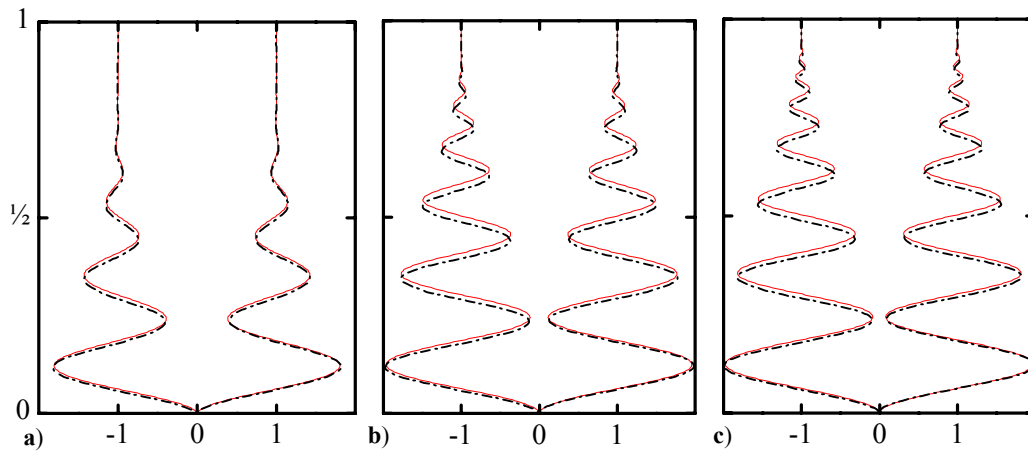
Figure 8. Comparing the asymptotic solution (full curves) to numerical computations of the nonlinear Navier-Stokes equations (chain curves) at two successive times. Here S = 25 , x/l = \frac{1}{2} , and m = 1 . Using a 40 \times 300 mesh resolution, simulation results are shown after 9 iteration cycles for (a) K = 10^4 , (b) K = 10^5 , and (c) K = 10^6 .
