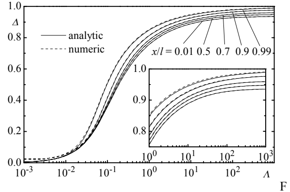
figure 10. Penetration depth for a wide range of parameters and axial locations including both numerical ( K = 10^6 ) and asymptotic predictions ( 10^4 < K < 10^8 ). Part of the graph is enlarged in the inset.
