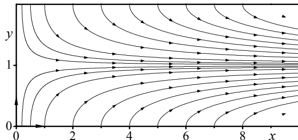
Figure 1- Two-dimensional mean flow streamlines.
